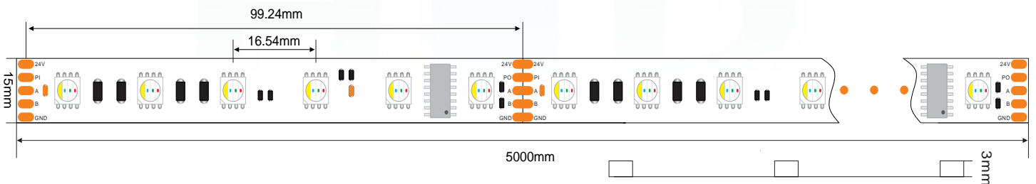
DC24V DMX512 RGBW 60led/m LED Strip
